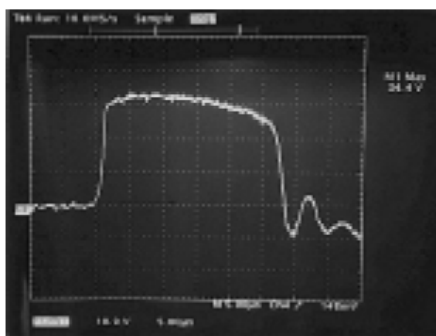
Shown here is a typical clamp voltage: MCG-12A suppression voltage is 34V
